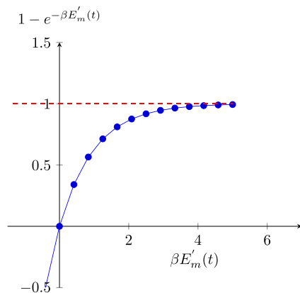
Fig. 5 Effect of control parameters (energy reservoir E'_m(t) and \beta ) on the regulation of compensation terms
