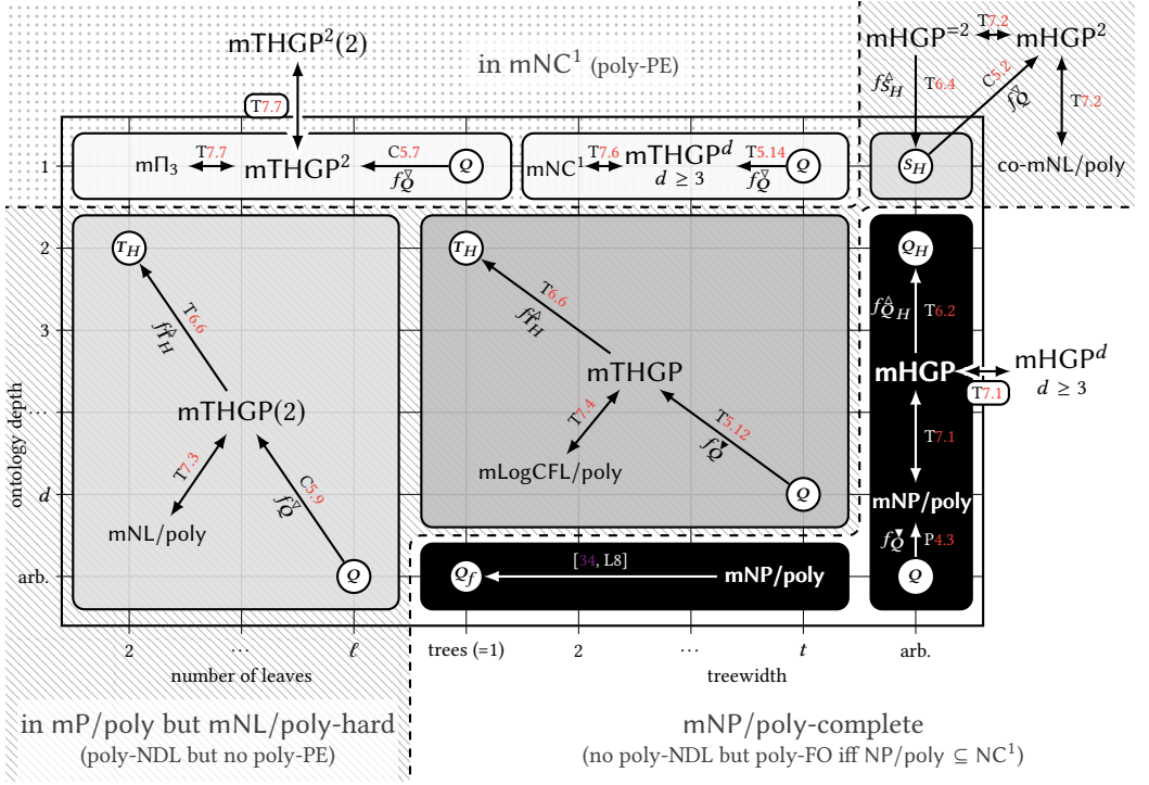
Fig. 19. Roadmap for the proofs of succinctness results.
