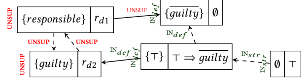
Figure 4: \mathcal{SG}_{\mathcal{KB}}^{BDL} of Example 6.
