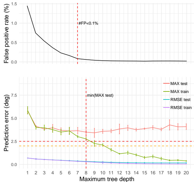
Fig. 4: Optimal max individual tree depth selection from false positive rate (top) analysis and training/test error (bottom).
