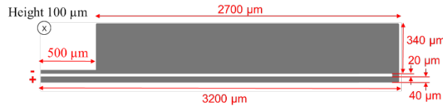
Fig. 12. Dimensions of the U-shaped electrothermal actuator.
