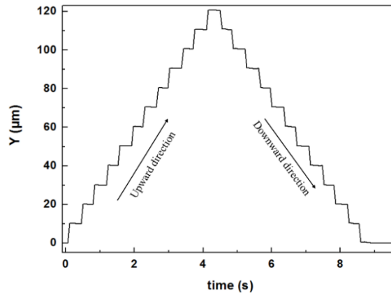
Fig. 20. Positions of the multistable actuator reached during 12 upward steps followed by 12 downward steps.
