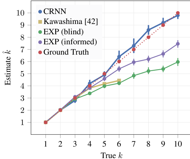
Figure 6: Average responses from humans ( EXP and Kawashima [42]) compared to our proposed CRNN. Error bars show 95% confidence intervals.
