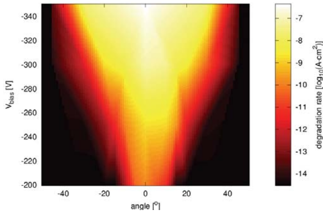
Figure 5. The heat map of the degradation rate as functions of tilting angle (abscissa) and the bias voltage (ordinate) obtained for 1217-MeV Xe-ion beam. Black color corresponds to the area, where no degradation is observed.
