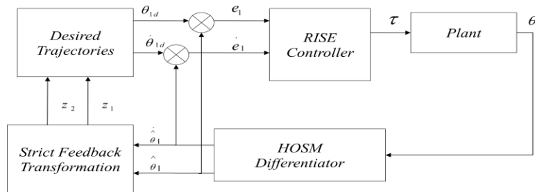
Figure 2. View of the block diagram of the proposed control approach
