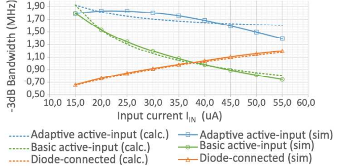
Figure 6. Cut-off frequencies versus input currents for the three compared types of current mirror
