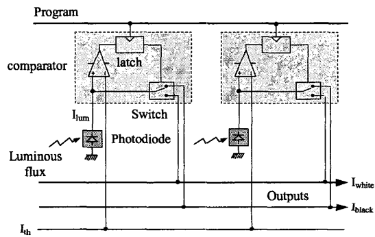
Figure 5: Block diagram of a programmable pixel
