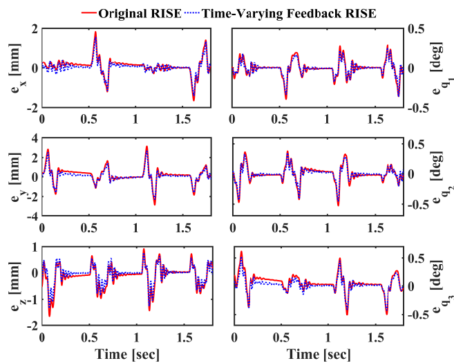
Fig. 3. Scenario 1: Evolution of the Cartesian and joint tracking errors.
