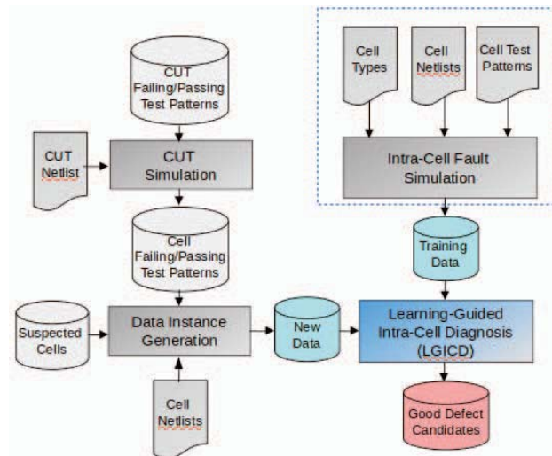
Figure 1: Learning-guided intra-cell diagnosis flow
