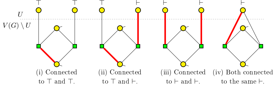
Figure 8: First cases of C_4^2 . The vertices of A \cap U labeled \perp are treated in the same way than vertices labeled \top . If both are connected to the same vertex labeled \top , the case depicted in subfigure (i) applies.
