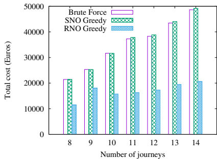
Fig. 4: Comparison with optimal scheduling plans.
