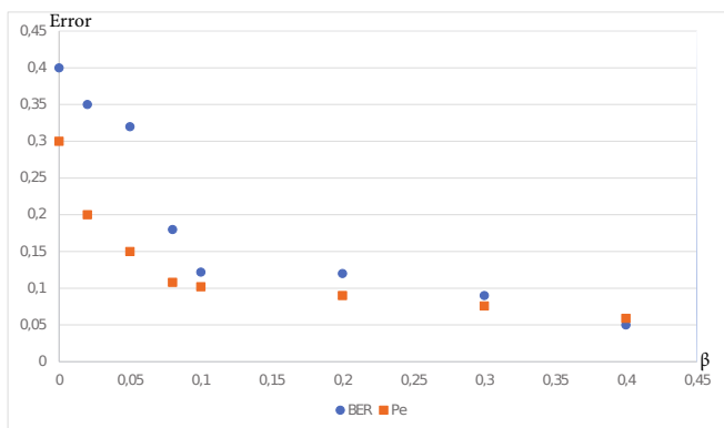
Fig. 9: BER and Pe for the second architecture for a payload size of 0,4 bpp in function of change rate \beta .
