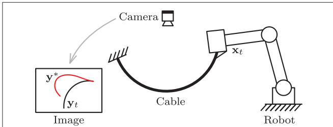
FIGURE 3 | Representation of the cable manipulation case of study, where a vision sensor continuously measures the cable's feedback shape \mathbf{y}_t , which must be actively deformed toward \mathbf{y}^* .
