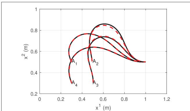
FIGURE 4 | Various configurations of the visually measured cable profile (black solid line) and its approximation with Fourier series (red dashed line).
