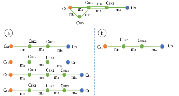
Figure 9: Derivation algorithm: all paths vs. Algorithm 2.
