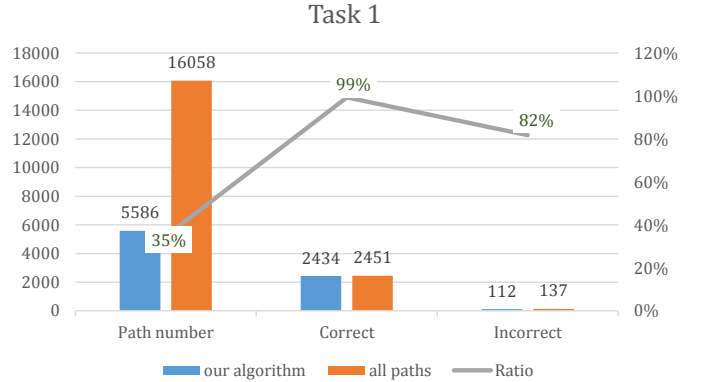
Figure 12: Task 1: derivation strategy comparison.
