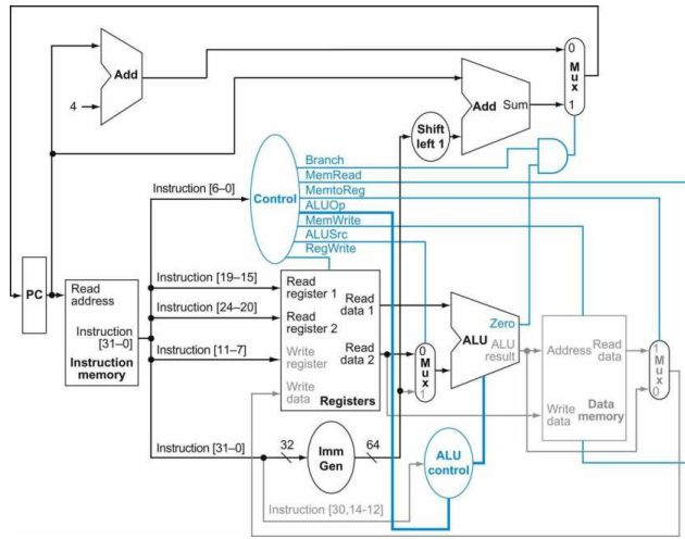
Figure 4: RISC-V overview [12]
