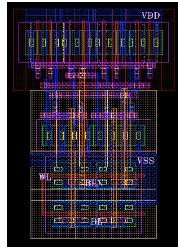
Fig. 8. Layout of the proposed S8P4N cell.
