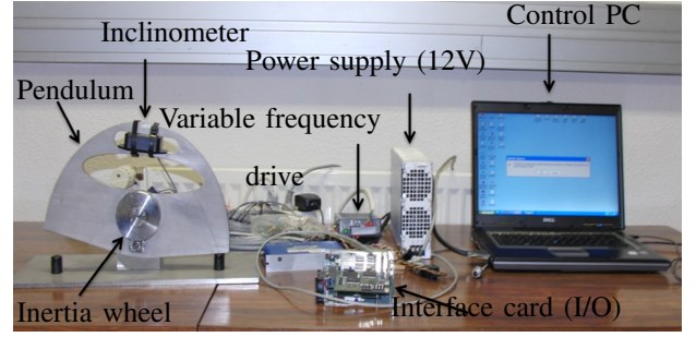
Fig. 3: View of the IWIP experimental testbed
