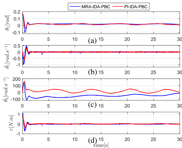
Fig. 7: Obtained experimental results for scenario 2: Persistent disturbance rejection. (a): Pendulum angular position, (b): Pendulum angular velocity, (c): Velocity of the inertia wheel, (d): The control input.
