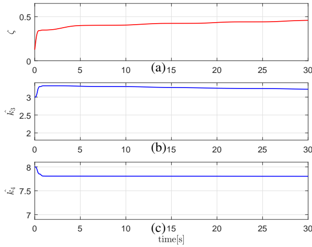
Fig. 5: Obtained experimental results for scenario 1: Nominal case. (a): The time evolution of \zeta , (b): The time evolution of \hat{K}_3 , (c): The time evolution of \hat{K}_4 .
