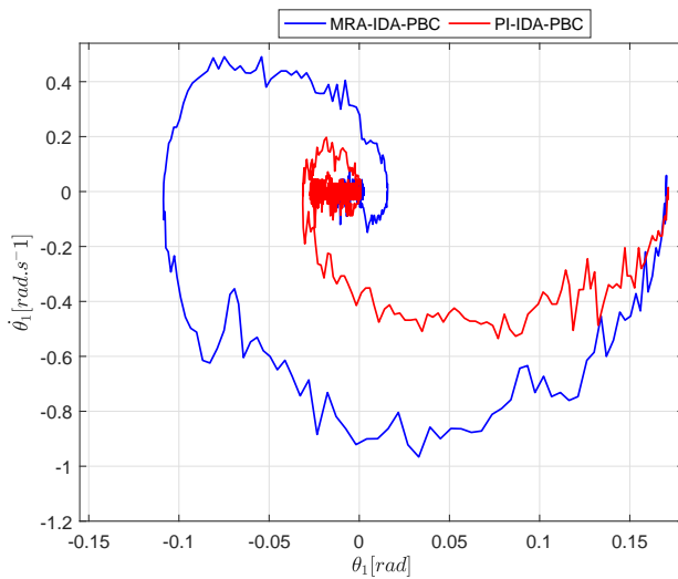
Fig. 6: Phase portrait (\theta_1, \dot{\theta}_1) for scenario 1.
