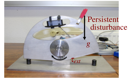
Fig. 2: Illustration of the external disturbance action applied on the pendulum body during experiments.
