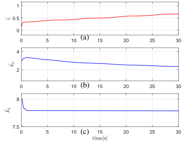
Fig. 8: Obtained experimental results for scenario 2: Persistent disturbance rejection. (a): The evolution of \zeta , (b): The evolution of \hat{K}_3 , (c): The evolution of \hat{K}_4 versus time.
