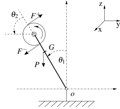
Fig. 1: Schematic view of the inertia wheel inverted pendulum.
