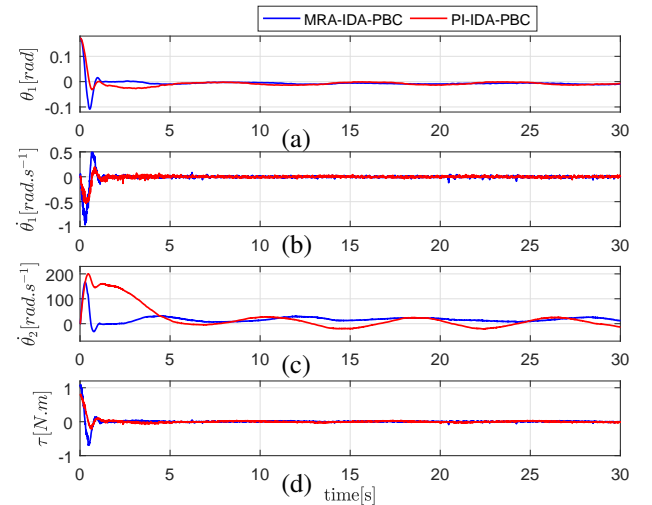
Fig. 4: Obtained experimental results for scenario 1: Nominal case. (a): Pendulum angular position, (b): pendulum angular velocity, (c): velocity of the inertia wheel, (d): The control input.
