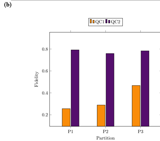
Figure 11: Results of the motivational example. (a) Circuit information and output fidelity results of different partitions. n: qubit number. g: gate number of the circuit. (b) Output fidelity results of different partitions.
