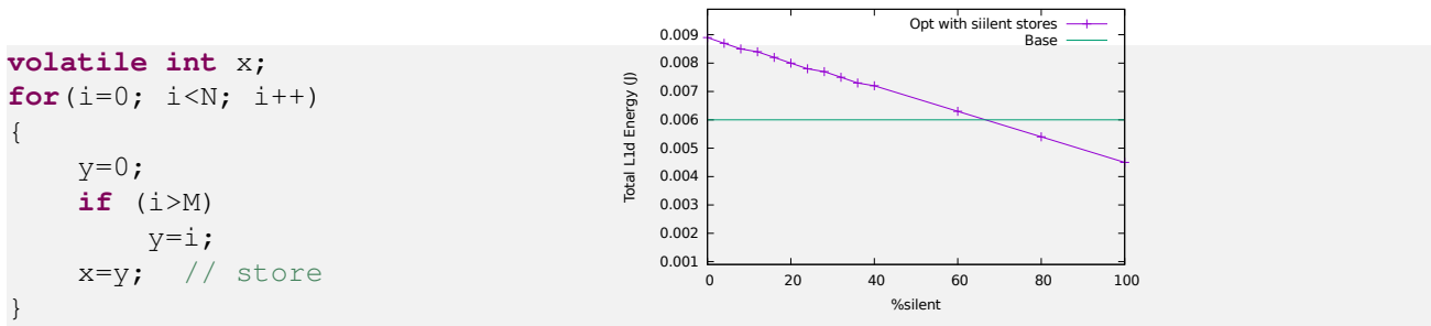
Figure 8: Determination of the profitability threshold of silent store elimination.
