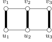
Fig. 11: Tightness of the approximation ratio for the cut-score greedy algorithm. Matching edges are bold. The approximation algorithm for the cut score provides a solution \{v_1, v_2, u_2, u_3\} whereas an optimal solution is \{v_2\} .
