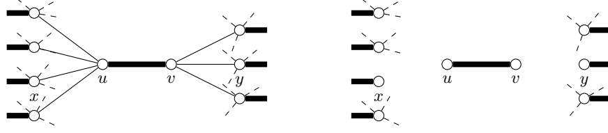
Fig. 10: A forbidden path xuvy (left) and the result of cutting all its vertices (right).
