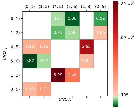
Fig. 1: The SRB result of IBM Q 7 Casablanca. The number represents the ratio of correlated error to independent error. Note that the SRB experiment is performed on CNOTs that can be executed in parallel, which means they do not share the same qubits. There are no SRB experiments on blank spots due to the sharing qubits.
