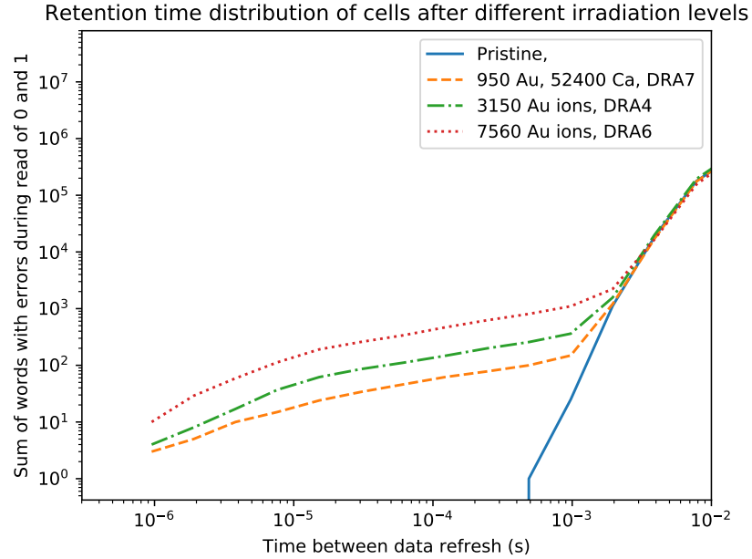
Fig. 6. Number of words containing stuck bits at different values of refresh time. The different curves shows the different memories that has been subject to a different number of ions on the cell arrays.
