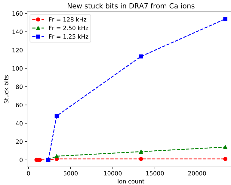
Fig. 4. Number of stuck bits in memory DRA7 as a function of cumulative fluence of Ca ions. Irradiation and post irradiation treatment to find the stuck bits done at F_{op} = 100 MHz, and with F_r = 128 kHz (red), F_{r,min} = 2500 Hz (green), and F_{r,min}/2 = 1250 Hz (blue).
