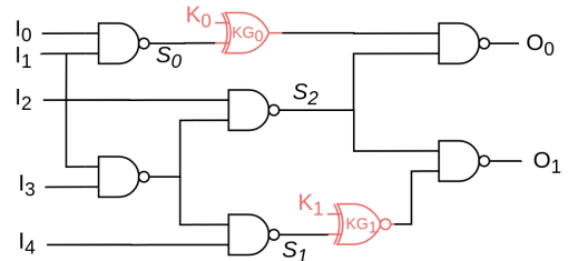
Fig. 1: Key-gate insertion based logic locking ( K_0K_1 = 01 ).
