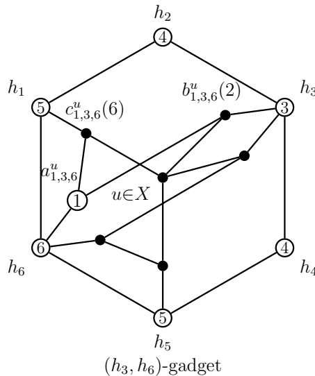
Figure 8: Situation where f(h_i) = i for every i \in \{3, 4, 5, 6\} .
