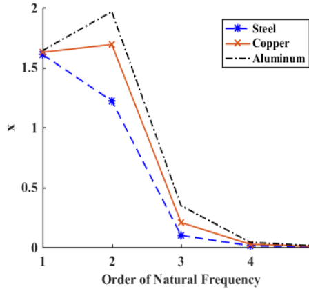
Fig. 5. Index values with three different material in the first five orders of natural frequency.
