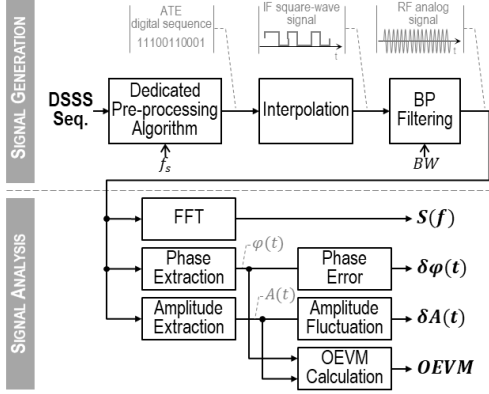
Fig. 6. Simulation setup
