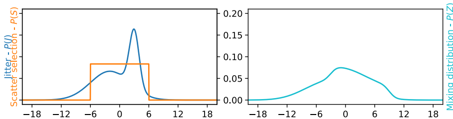
Figure 1: Effect of a Scatter window on a mixture subject to arbitrary jitter. (left) Probability distributions of jitter and Scatter selection. (right) Resulting mixing distribution, i.e. distribution of mixing variable Z .
