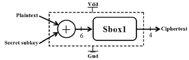
Figure 4. Sub-module of DES cipher.
