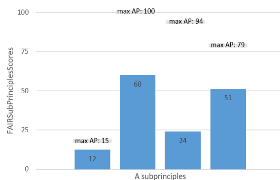
Fig. 10. Average normalized FAIRSubPrincipleScore for R.
