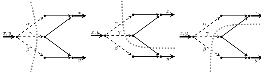
Figure 4: Network information transmission problem that corresponds to Gray–Wyner profile.
