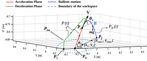
Fig. 3. Illustration of the pick and throw motion consisting of robot motion acceleration and deceleration phases together with the ballistic motion of the thrown object.
