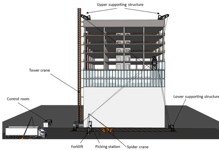
Fig. 29. Future performance of the Hephaestus robot on a construction site.
