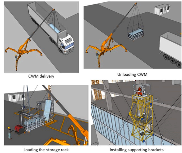
Fig. 29. Future performance of the Hephaestus robot on a construction site.
