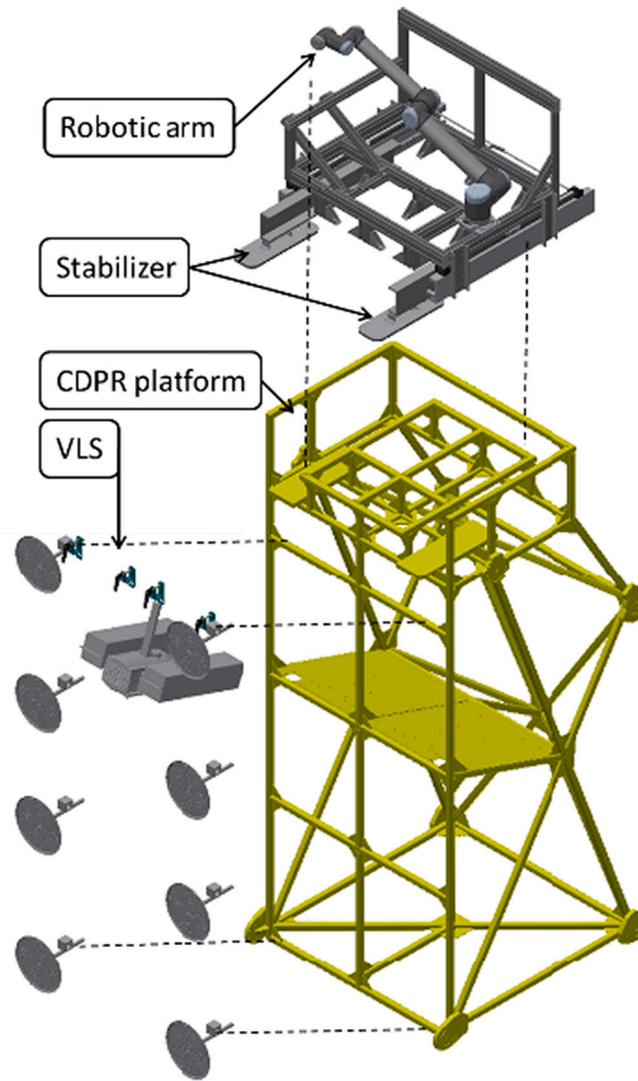
Fig. 17. View of the MEE on top of the CDPR platform during the first demonstrator (top), exploded view of the front side (bottom).
