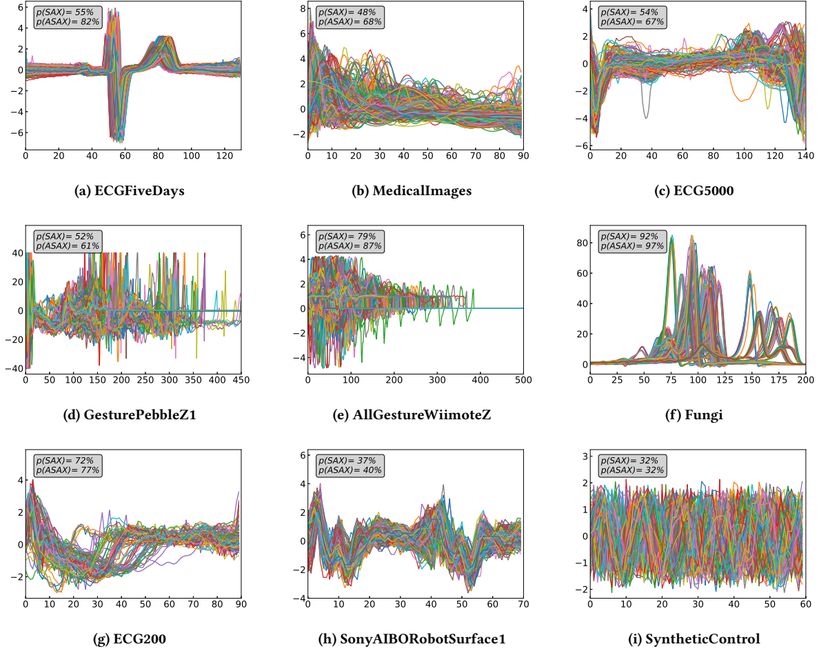
Figure 6: The data distribution of the tested datasets, and the precision results for each dataset. p(\text{SAX}) and p(\text{ASAX}) show the precision of SAX and ASAX respectively. The datasets are sorted in descending order of precision gain.
