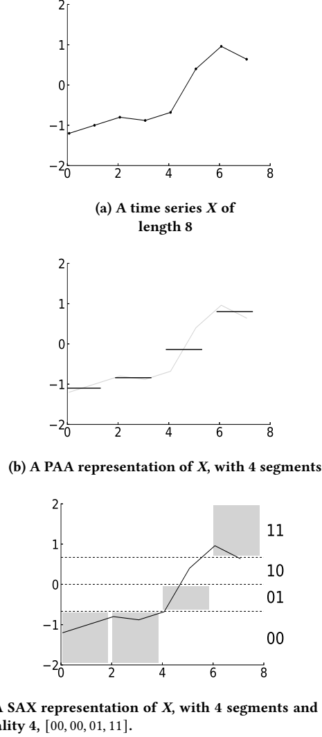
Figure 2: A time series X is discretized by obtaining a PAA representation and then using predetermined break-points to map the PAA coefficients into SAX symbols. Here, the symbols are given in binary notation, where 00 is the first symbol, 01 is the second symbol, etc. The time series of Figure 2a in the representation of Figure 2c is [first, first, second, fourth] (which becomes [00, 00, 01, 11] in binary).
