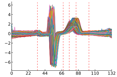
(b) ASAX segmentation on D , with 6 segments
