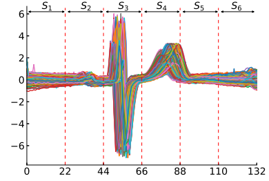
(a) SAX segmentation on D , with 6 segments
