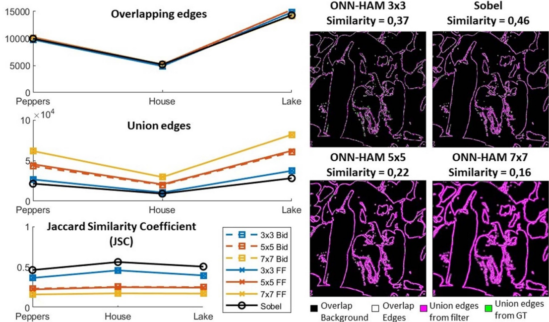
Figure 13. Number of overlapping edges, union edges, and similarity coefficient between our ONN solutions simulated on Matlab, Sobel state-of-the-art and Canny GT reference on large scale black and white images Peppers , House , and Lake . Similarity outputs of the bidirectional ONN solutions simulation on Matlab and Sobel solution compared to Canny on black and white Peppers image.
