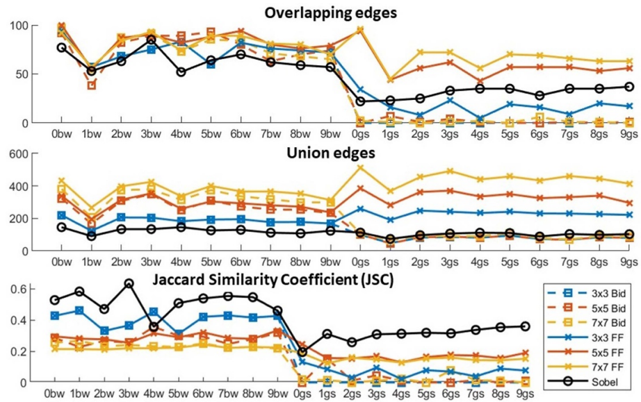
Figure 10. Number of overlapping edges, union edges, and similarity coefficient between our digital ONN solutions and Canny reference, and between Sobel state-of-the-art and Canny reference on MNIST black and white (bw) and grayscale (gs) digit images.
