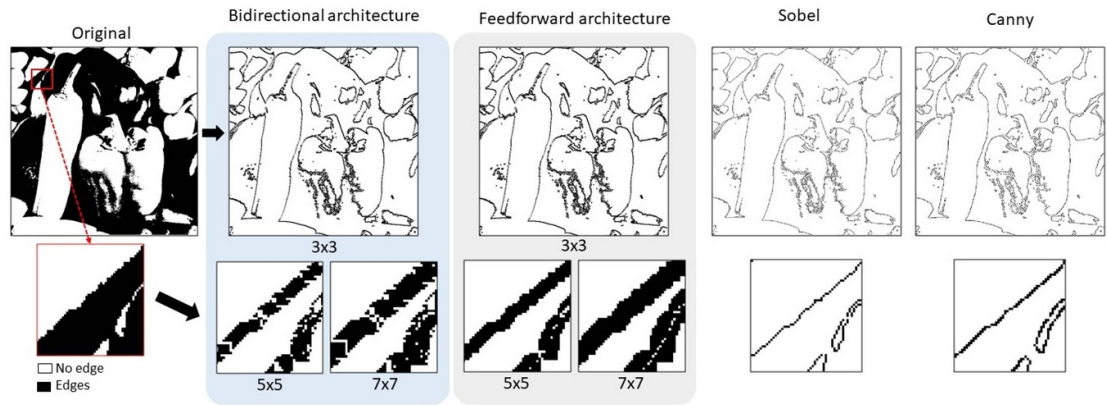
Figure 12. Edge detection results of the digital ONN designs for the bidirectional architecture with input size 3 \times 3 , 5 \times 5 , and 7 \times 7 , and for the feedforward architecture with input size 3 \times 3 , 5 \times 5 , and 7 \times 7 , compared with previous work [21] and state of the art on the black and white 512 \times 512 standard 'pepper' image.
