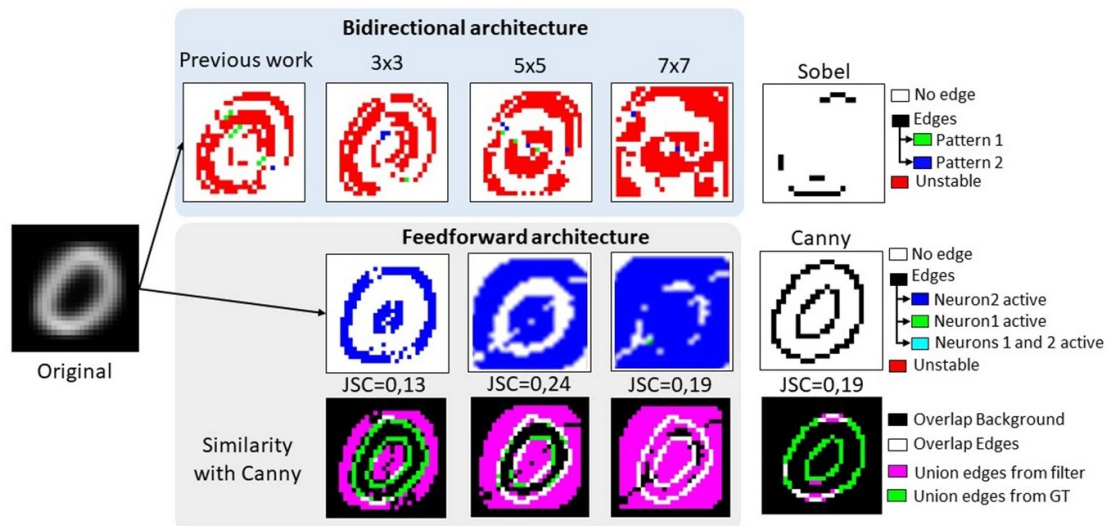
Figure 11. Edge detection results of the digital ONN designs for the bidirectional architecture with input size 3 \times 3 , 5 \times 5 , and 7 \times 7 , and for the feedforward architecture with input size 3 \times 3 , 5 \times 5 , and 7 \times 7 , compared with previous work [21] and state of the art Sobel and Canny on a gray scale 28 \times 28 MNIST image.
