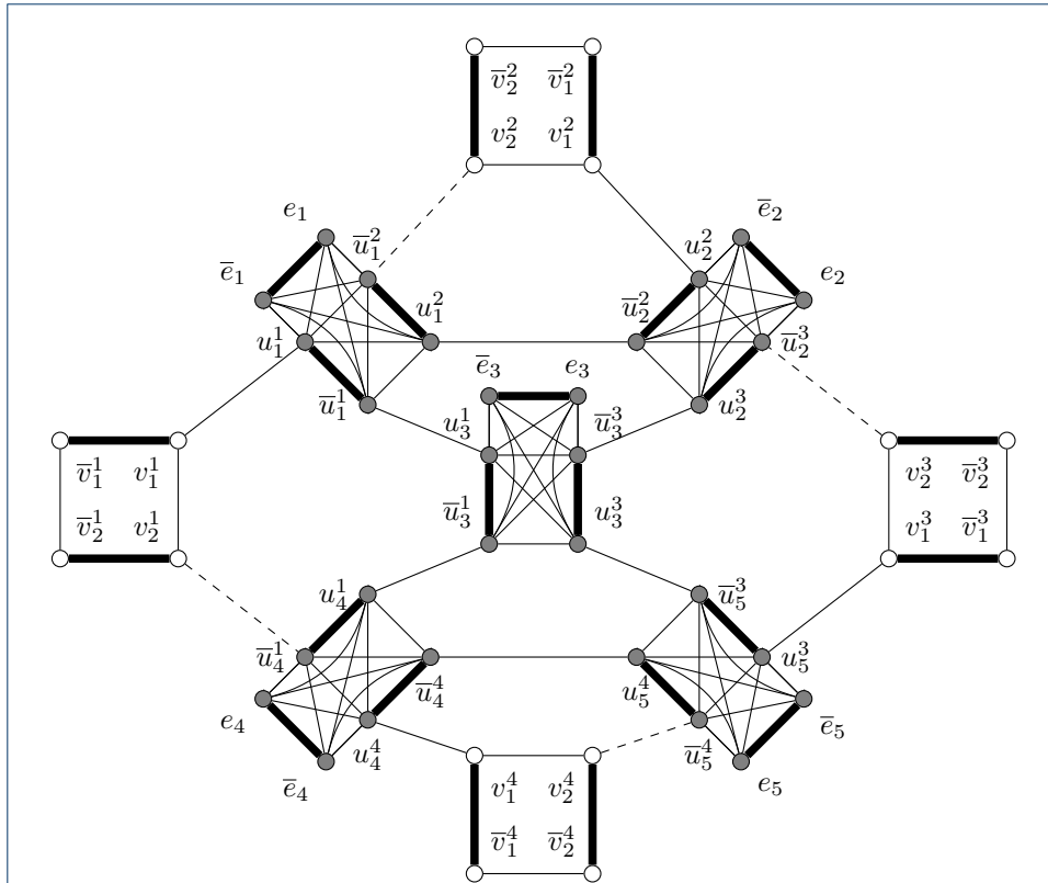
Figure 4: Example of a scaffold graph produced by Construction 2. The input graph is composed by the edges e_1 = v_1v_2 , e_2 = v_2v_3 , e_3 = v_1v_3 , e_4 = v_1v_4 and e_5 = v_3v_4 . Gray vertices in the figure belong to an edge gadget and white vertices belong to a vertex gadget. Matching edges are bold. Solid edges have weight zero and dashed edges have weight one. The long vertex-cycle C(v_2) corresponds to the vertices \{\bar{v}_1^2, v_1^2, u_2^2, \bar{u}_2^2, u_1^2, \bar{u}_1^2, v_2^2, \bar{v}_2^2\} .
