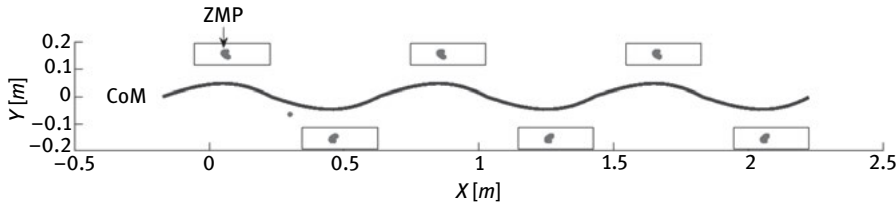
Fig. 16. Evolution of ZMP and CoM trajectories with the proposed optimal 3MLIPM.
