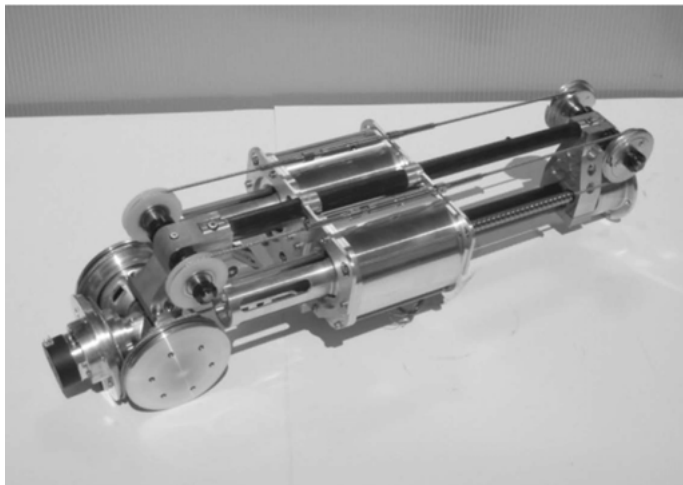
Fig. 5. View of a real manufactured module.
