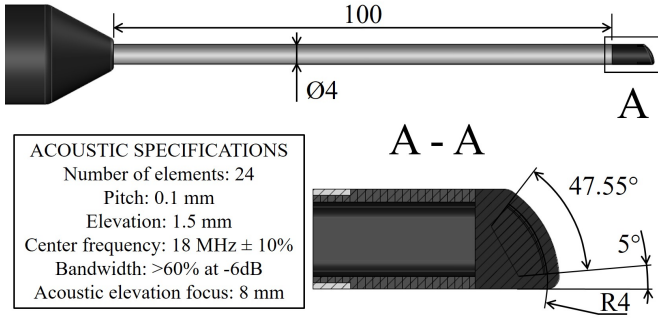
Fig. 1: Technical specifications of the miniaturized endoscopic 2D US transducer. Distances are expressed in mm.
