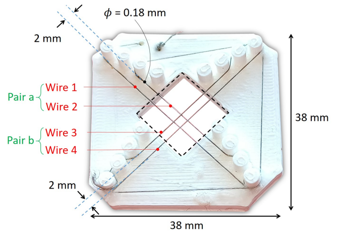
Fig. 5: Top view of the 3D printed phantom used for evaluating the accuracy of the reconstruction procedure.
