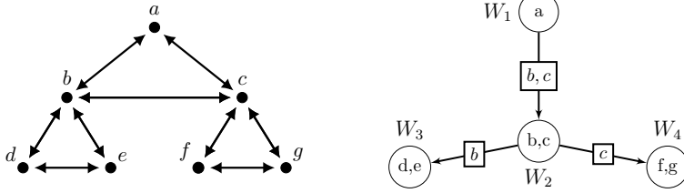
Fig. 4: A digraph D and an arboreal decomposition of D of width two. A bidirectional edge is used to represent a pair of edges in both directions.
