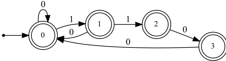
FIGURE 1. Automaton recognizing the valid representations.
