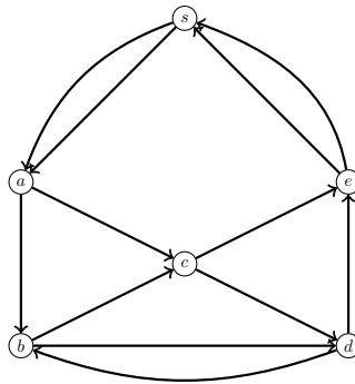
Figure 12: A 2-arc-strong multigraph D with \alpha(D) = 2 and no pair of arc-disjoint branchings B_s^+, B_s^- .
