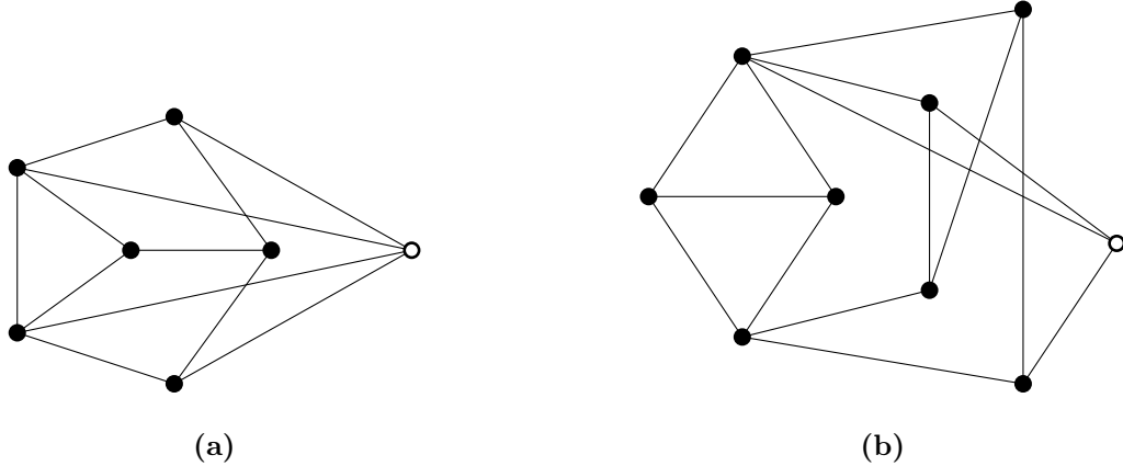
Figure 2: Not every graph obtained from a planar graph with at most one triangle by adding a 4-vertex is 3-colorable (example (a)), nor is a graph obtained from a planar graph with two triangles by adding a 3-vertex (example (b)). The added vertex is depicted with an empty disk in both cases.
