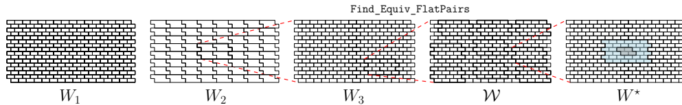
■ Figure 2 Sequence of walls in the general scheme of our algorithm. The first wall is obtained by applying the algorithm of [72, Proposition 14] for the wall W_0 in the input graph G .
