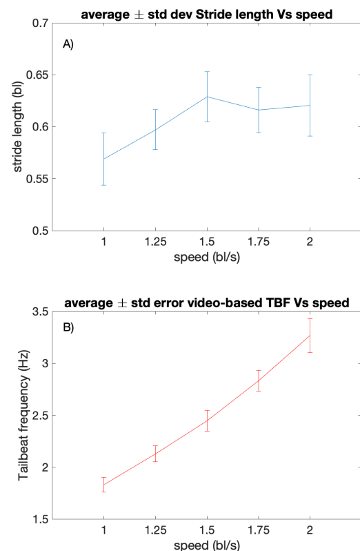
Figure 4. (A) stride length (bl) versus water speed (bl/s), (B) video-based estimation of TBF (Hz) versus water speed (bl/s) at 5 water speeds.
