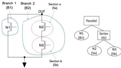
Fig. 8. Generic NMOS network and its corresponding structure tree.
