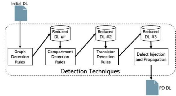
Fig. 10. Detection techniques flow of the new version of TrUnDeL.
