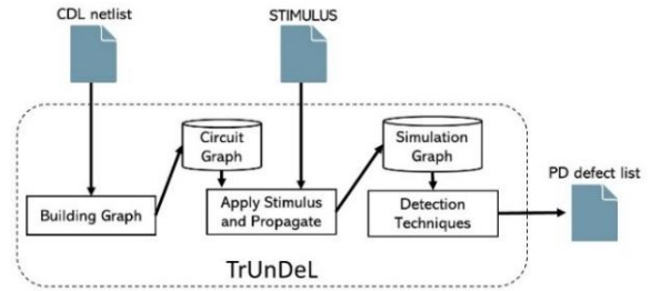
Fig. 2. TrUnDeL flow.
