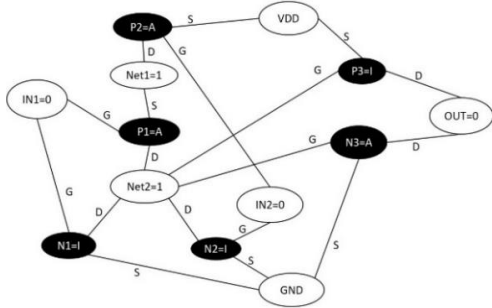
Fig. 4. OR Simulation Graph.
