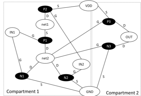
Fig. 3. OR Circuit Graph.
