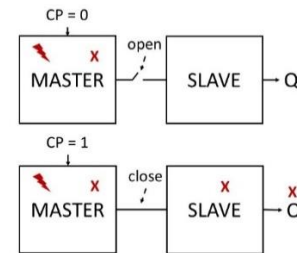
Fig. 7. Defect propagation between cycles and subcycles example.
