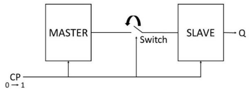
Fig. 5. General sequential cell configuration.
