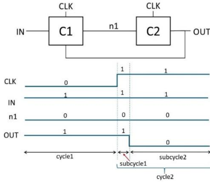
Fig. 6. Feedback loop causing a glitch.
