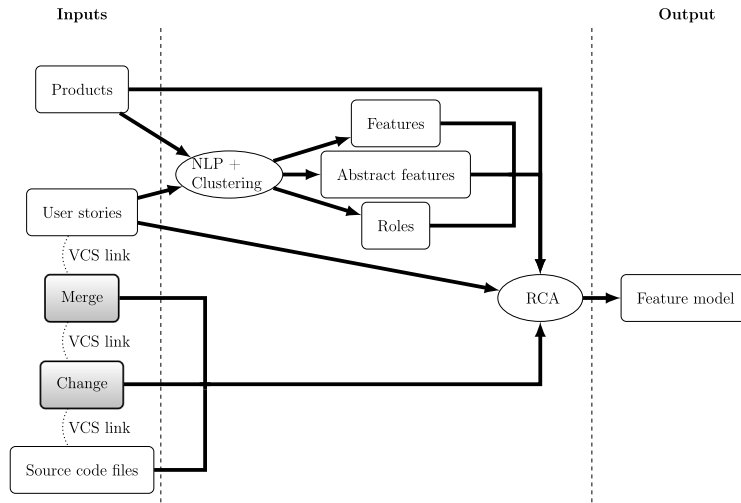
Fig. 2. Process Overview: Automated process from products, user stories linked to the source code via VCS links (inputs) to the feature model (output) using NLP, clustering, and RCA. Rectangle boxes represent artifacts, while ellipses represent processes. Grey boxes indicate artifacts originating from the VCS.
