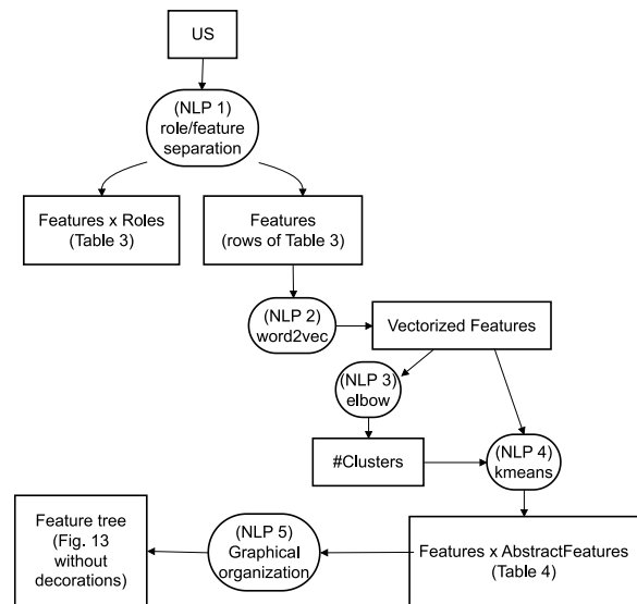
Fig. 4. NLP and clustering steps: user stories are separated into role and feature parts (NLP 1); word2vec is applied to features (NLP 2); resulting vectorized features are analyzed with elbow to compute a cluster number (NLP 3); k-means is applied to obtain abstract features (NLP 4); the features (including abstract ones) are used to draw the skeleton of the feature model, i.e. the feature tree (NLP 5).
