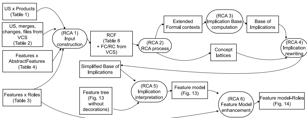
Fig. 15. Summary of the RCA part.
