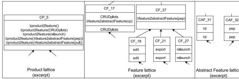
Fig. 11. Excerpt of the concept lattices for products, features and abstract features produced by RCA after simplification of the relational attributes.
