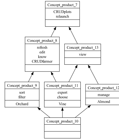
Fig. 8. Concept lattice of the formal context of Table 6.
