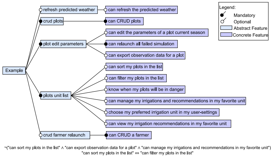
Fig. 13. Feature model example.
