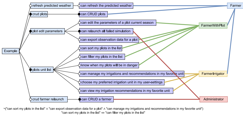
Fig. 14. Enhanced feature model (with additional colored roles and links).
