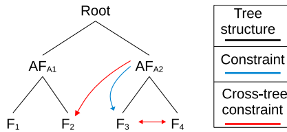
Fig. 12. Feature tree with constraints.
