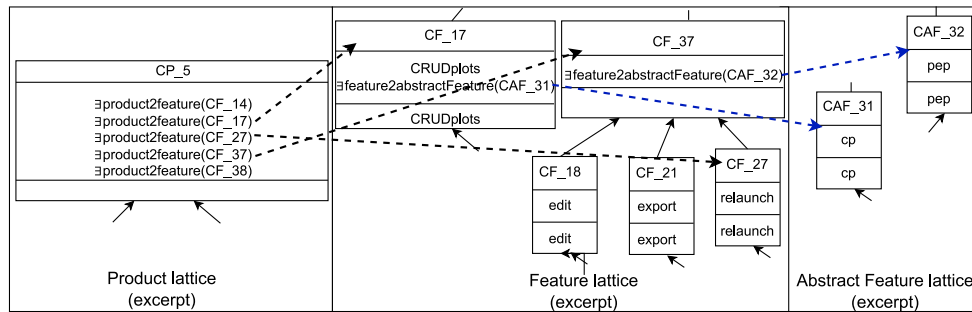
Fig. 10. Excerpt of the concept lattices for products, features and abstract features produced by RCA. Dotted arrows (manually added on the figures produced by FCA4J) highlight the connections which are done between the concepts through the relational attributes.
