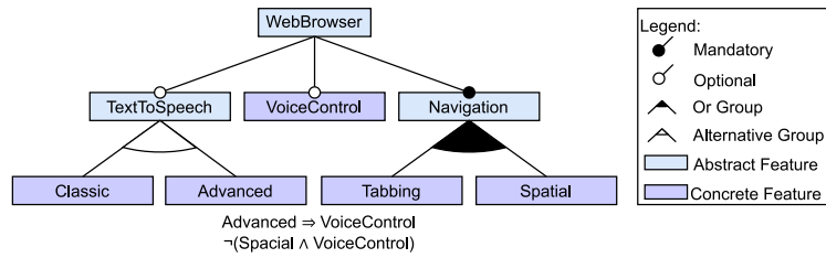
Fig. 1. An example of a feature model for a WebBrowser product line.
