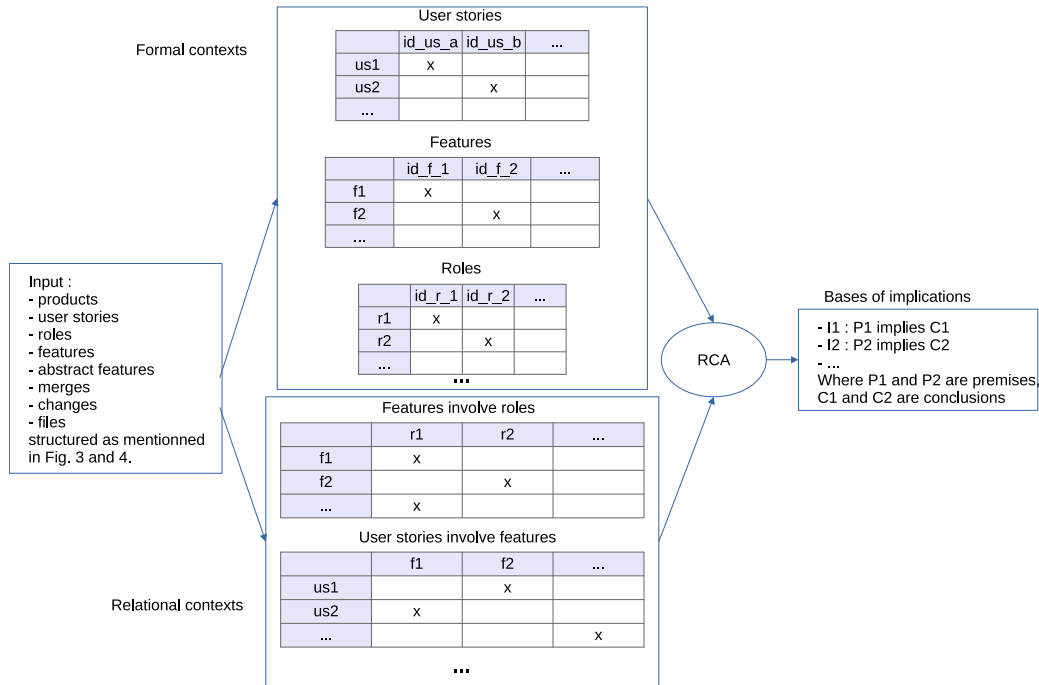
Fig. 7. Obtaining a base of implications using RCA.
