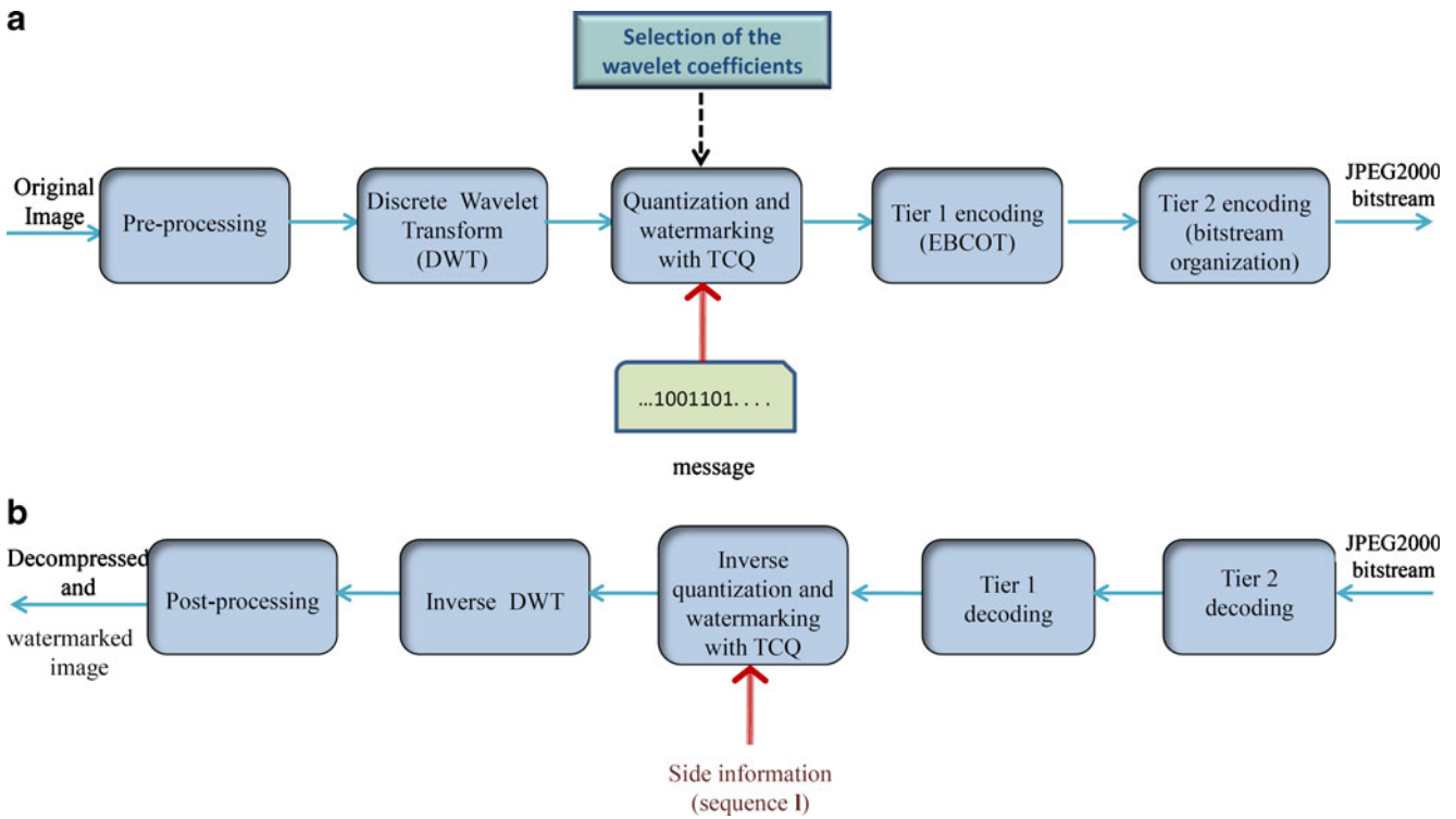
Fig. 4 The joint JPEG2000/watermarking scheme: a compression process, b decompression process
