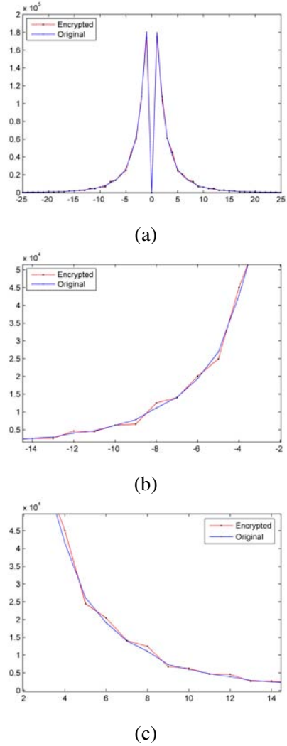
Fig. 18: Histograms of original and SE-CAVLC NZs: a) Complete graph, b) Zoomed graph of negative x-axis, c) Zoomed graph of positive x-axis.
